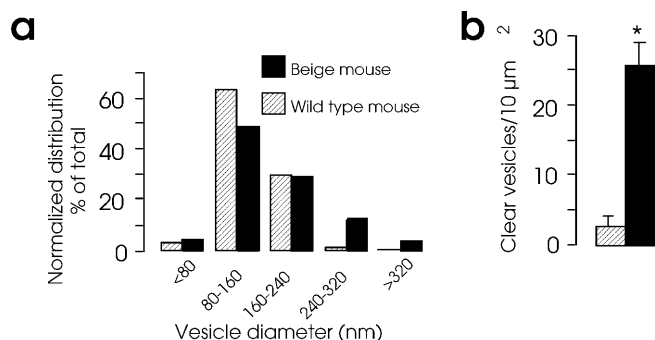
Fig. 2a, b Morphometric studies on chromaffin cell organelles. a Normalized CG size distribution in BM and control adrenal chromaffin cells. Abscissa shows the granule distribution at the ranges indicated. Diameters were measured from EM micrographs. b Clear vesicles >200 nm in diameter (means \pm SEM) counted from EM photographs (5 sections/gland; 4 mice of each type), obtained from adrenomedullary sections. * P > 0.01 Student's t -test
